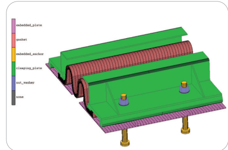
Fatigue Simulation
