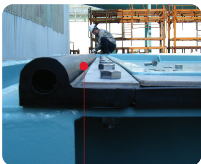
Side Seal
